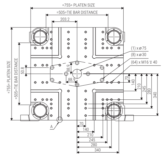
170 Ton Moving Plate
