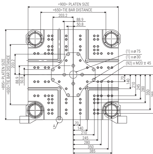
280 Ton Moving Plate
