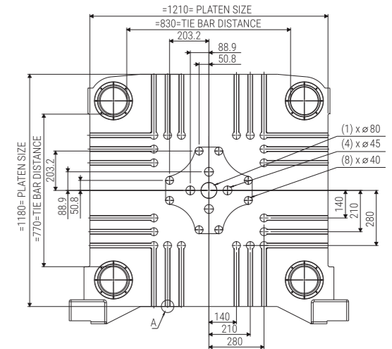
480 Ton Moving Plate
